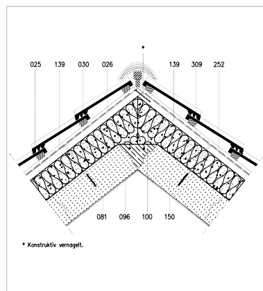
Regeldetail First
