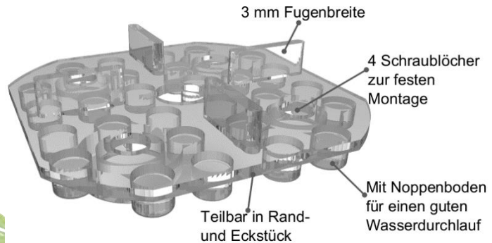
Abbildung 1: TK-U 3/10 (4Fugenstege)
